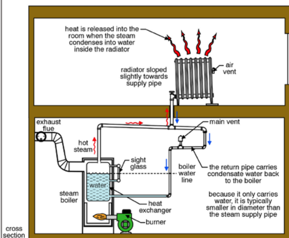
How steam systems work
