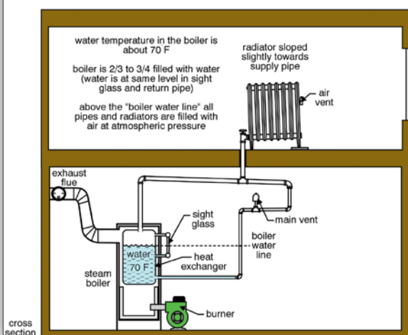
Steam system operation: at rest
