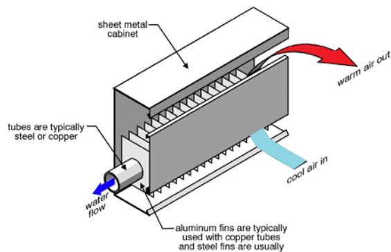
Finned tube baseboard
