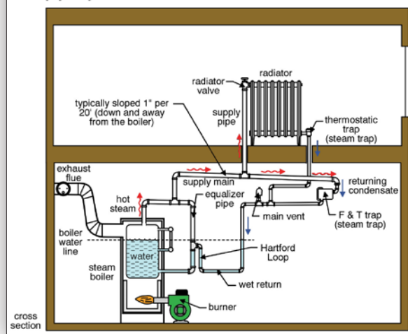
Two pipe system
