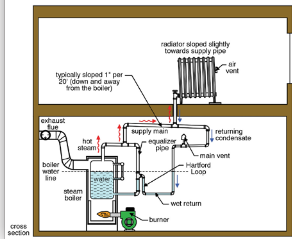
One pipe parallel flow system
