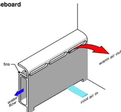
Cast iron baseboard
